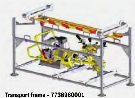
Transport frame - 7738960001
